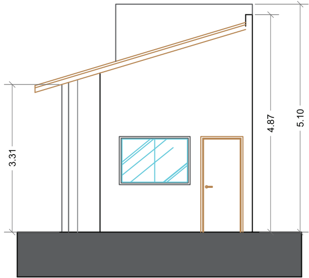
FACHADA PRINCIPAL
